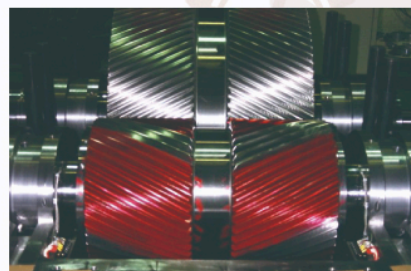
Turbine Compressor (High speed Gears)
